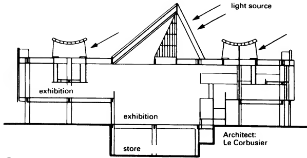
1 National Museum of Western Art, Tokyo: section
